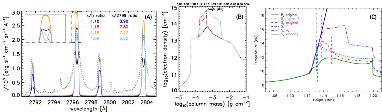
Figure 2. Illustrating the effect of increased electron density in the upper chromosphere on the Mg II NUV spectrum. Panel (A) shows the Mg II spectra synthesised from a RADYN simulation, using RH, where each colour represents a different modification to the electron density, the stratification of which is shown in panel (B). The black line is the original, and the dotted line is a sample observed flare spectrum from IRIS. The resonance to subordinate line ratios are indicated. An order of magnitude increase in the electron density to > 5 \times 10^{14} \text{ cm}^{-3} is required to produce a single peaked profile. Panel (C) shows that increasing the electron density (purple line, compared to all others) results in a stronger coupling to the Planck function (black line), hence the lack of central reversal in that instance. The vertical lines in that panel are the formation heights of the Mg II k line core for each model atmosphere. Figure adapted from Rubio da Costa and Kleint [2017]. ©AAS. Reproduced with permission.
